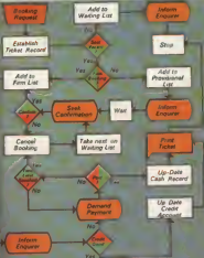
FLOW CHART FOR A FLIGHT BOOKING
